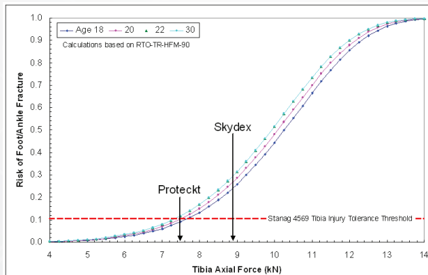
Stenag 4569 Tibia Tolerance Threshold Plot versus Peak Tibia Loading Change in Velocity of 7 (m/s) 5.9 (ms) Peak Load 304 G's 50th Percentile 180 Pound ATD.
